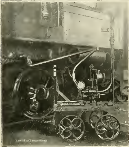
FIG. 1. WATER CHANGING APPARATUS CONNECTED TO LOCOMOTIVE BOILER.
